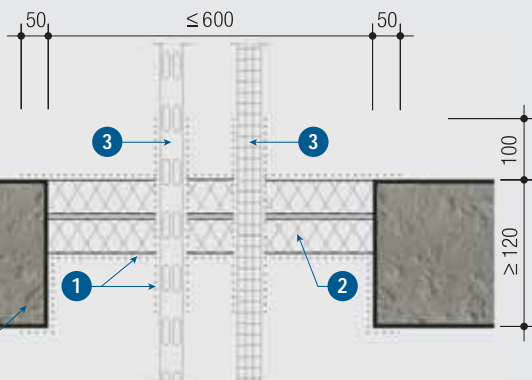
Detail 3 Floor penetration
